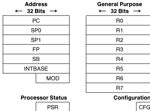
FIGURE 2-1. NS32CG16 Internal Registers
